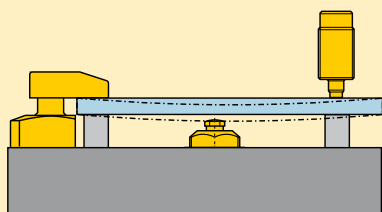
Figure 1 Simple hydraulic fixture with minimal workpiece deflection.
