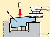
Figure 5b Incorrectly located workpiece
