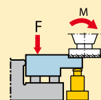
Figure 5c Correctly located workpiece
