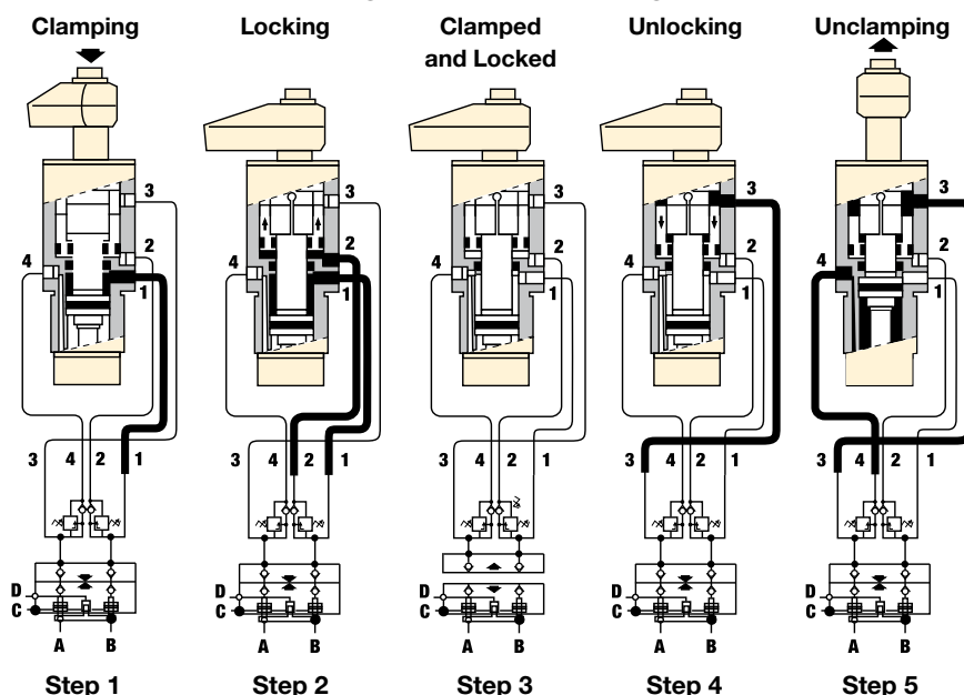
MPTR-100 Collet-Lok® swing cylinder
