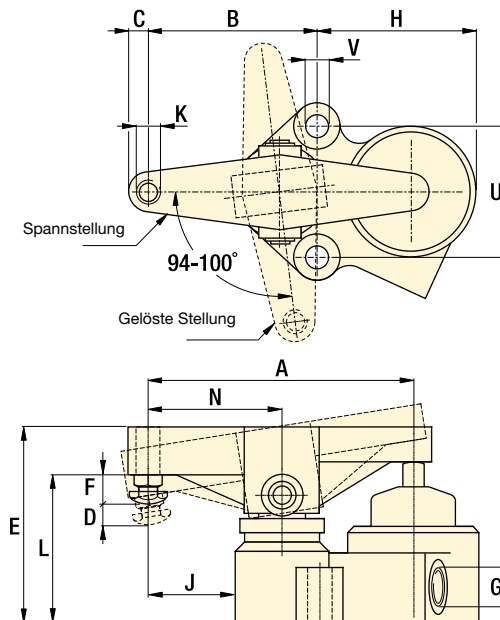
ASC-30, -100
