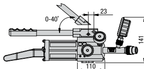
HP350/550/1000D
